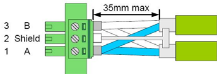
Figure 4-2 CNet cable pinouts
