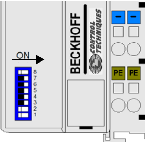
Figure 5-1 DIP switches
