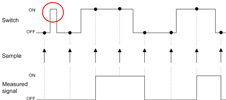
Figure 7-2 Aliasing example
