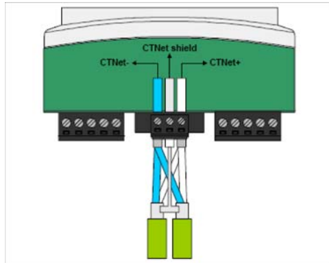
Figure 4-3 CTNet network connections
